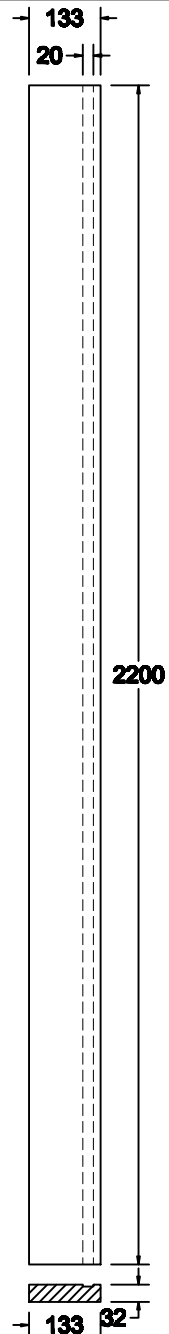
Frame 32 x 133 x 2200 mm
